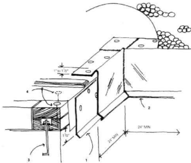
GRAVEL STOP
