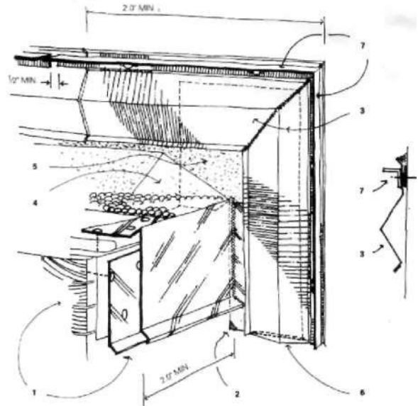
TYPICAL GRAVEL STOP TERMINAL
